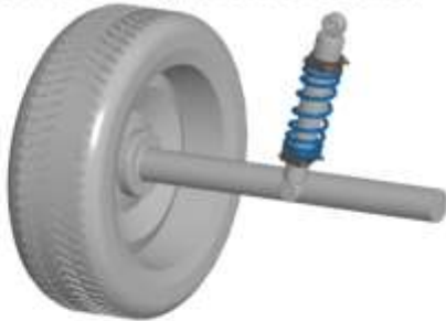
Auxiliary Coil Spring HV-.....3 mounted on original shock absorber
